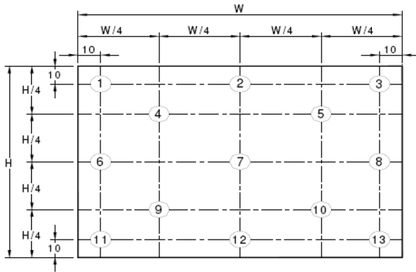
Fig8-1 Measuring point
